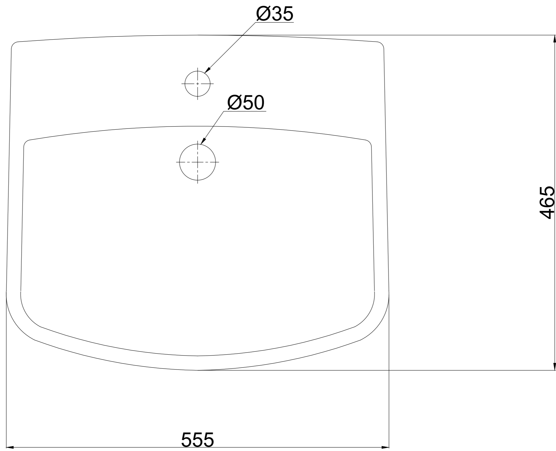
TOP VIEW
